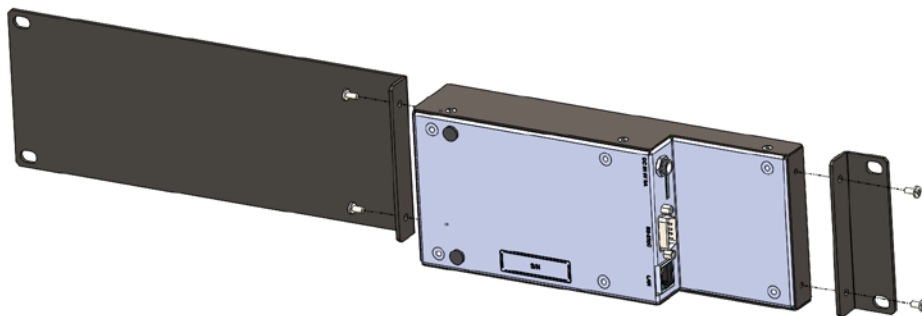
[Fig. 4] Attaching 701A05 and 701A06
