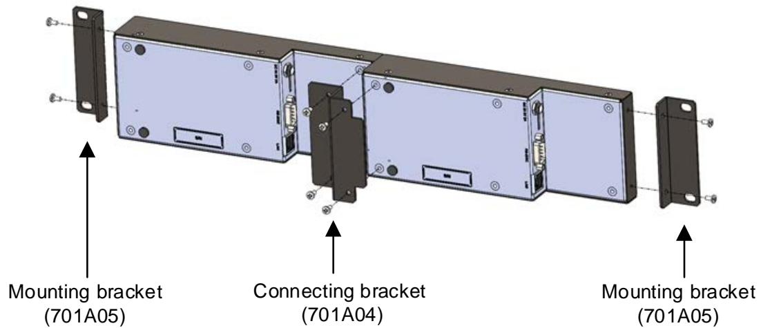
[Fig. 6] Attaching 701A04 and 701A05
